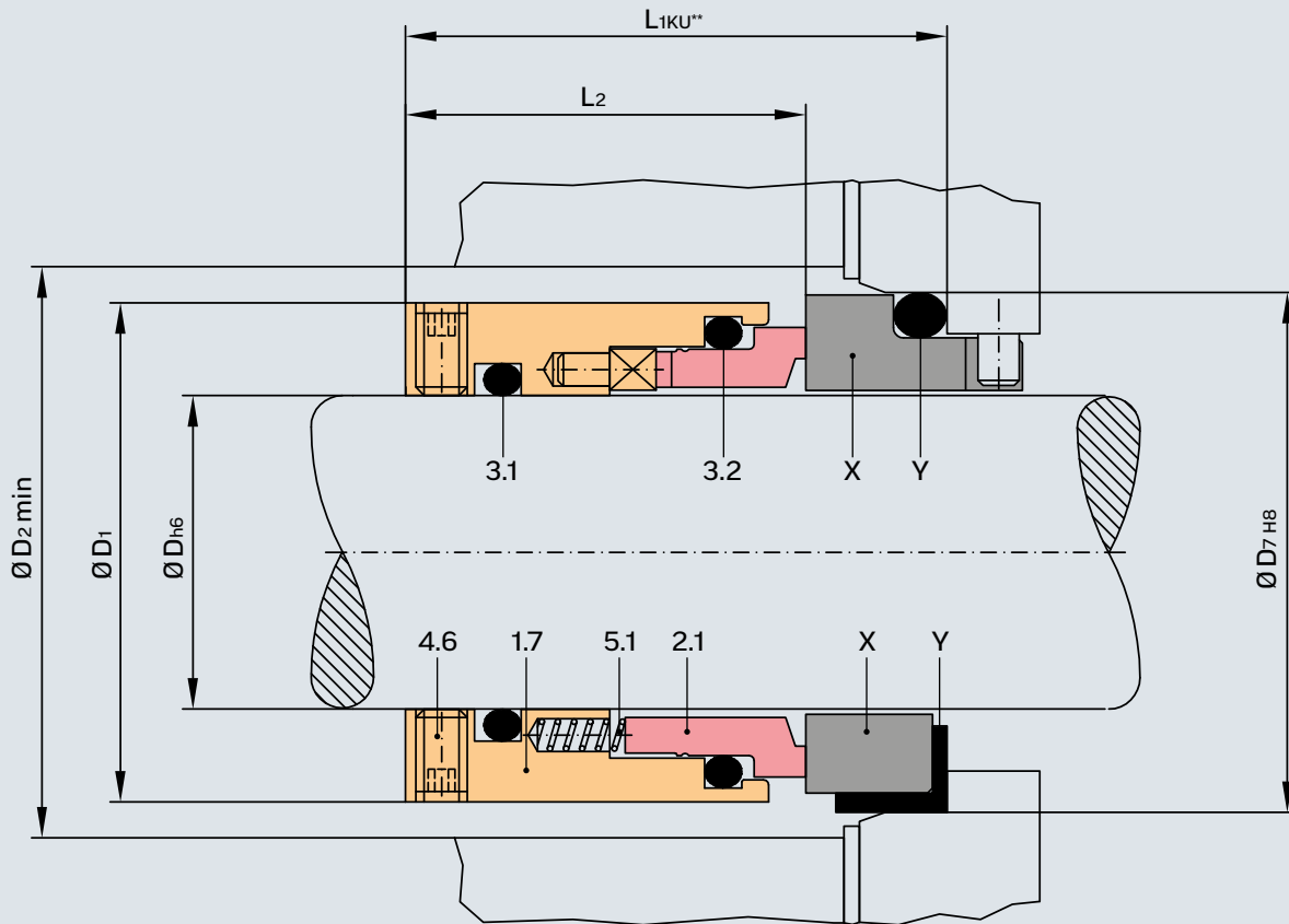
Dimension table Ø 16 - 100 millimetres
